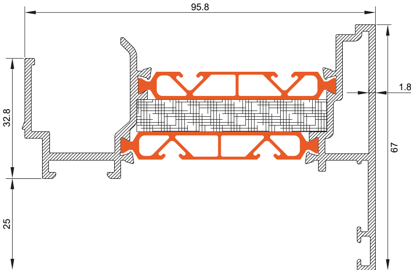
ADAPTER PROFILES
